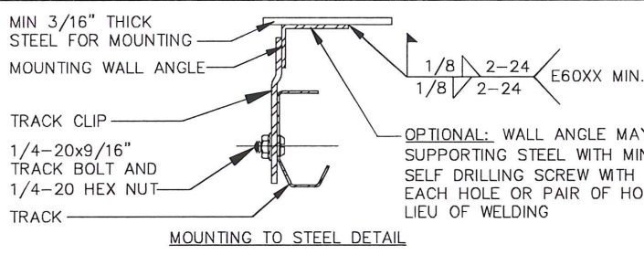
MOUNTING TO STEEL DETAIL
