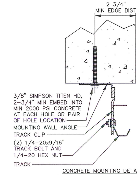
CONCRETE MOUNTING DETAIL
